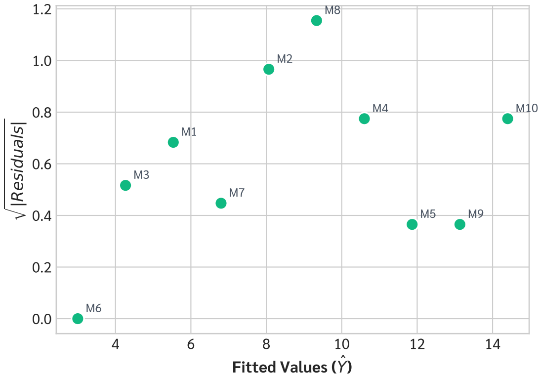
Scale-Location Plot
